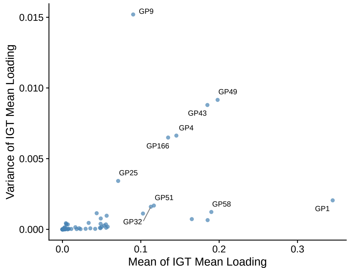
GP Mean of IGT Mean Loading vs. Between-IGT V
